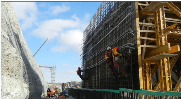
View of the exterior wall rebar and electrical conduit
