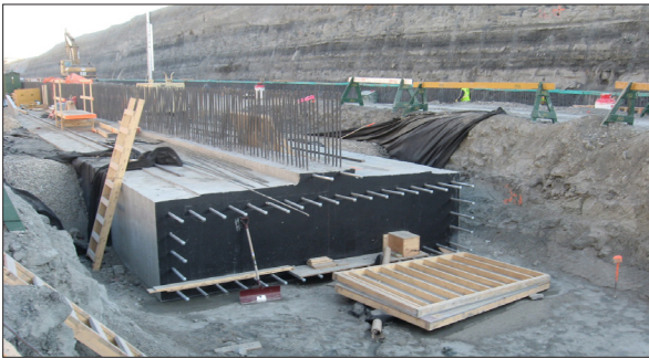
View of the central footing for the tunnel
